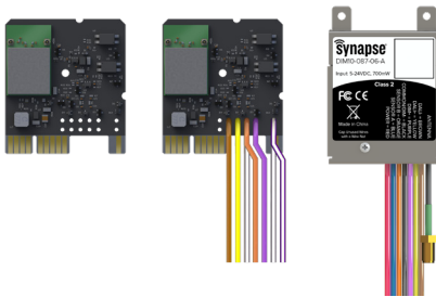
DIM10-087-06, DIM10-087-06-FW, and DIM10-087-06-A Embedded Light Controllers
